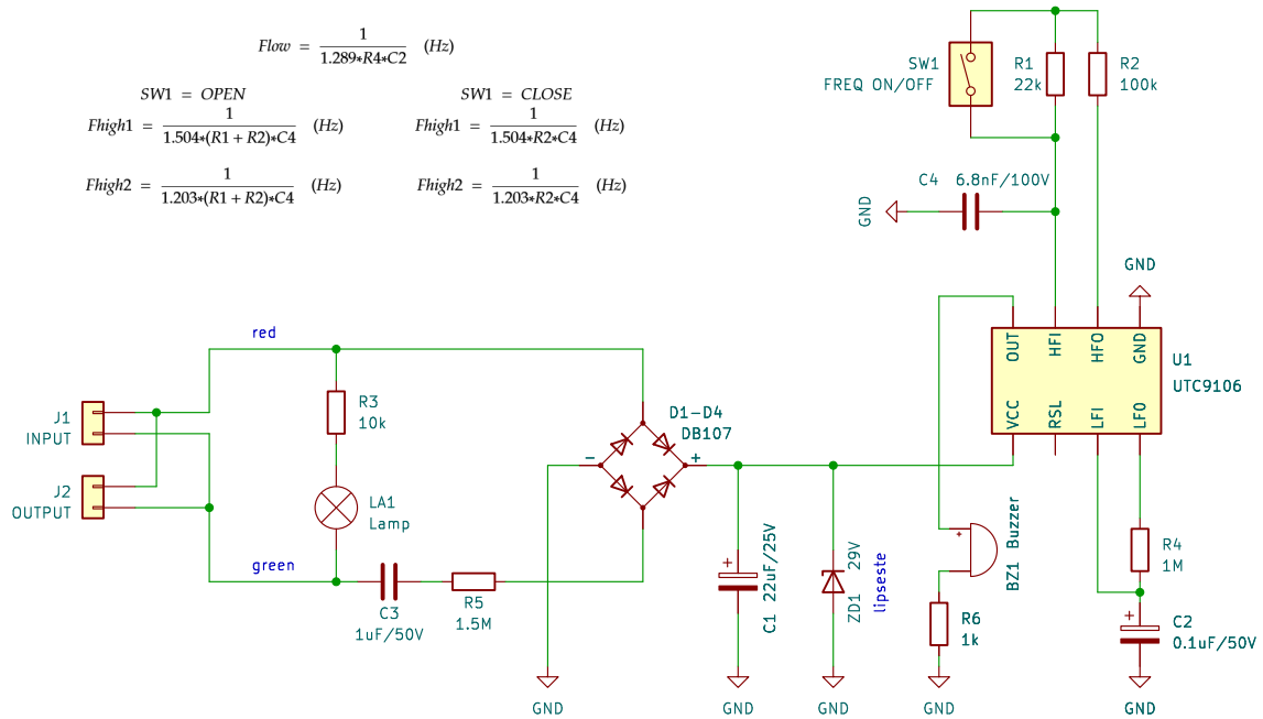
External telephone ringer JMX-102 using UTC9106
